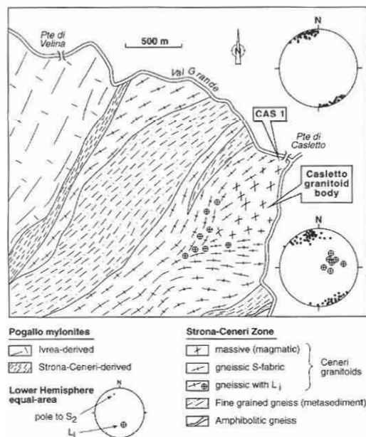
Fig. 6 Map of part of the Ceneri granitoid body at Ponte di Casletto (see Fig. 1 for location). Note trend of S2 schistosity in and around the granitoid body (see text for explanation). Intersecting S2 surfaces yield an intersection lineation, L1. CAS1 is sample of gneissic Ceneri granitoid dated by KÖPPEL and GRÜNENFELDER (1971). Map from figure 2.02 in HANDY (1986).
