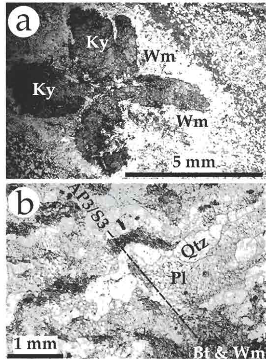
Fig. 4 Microstructures: (a) Chiasolite (viewed perpendicular to its long axis) replaced by kyanite (Ky) that is rimmed by white mica (Wm); sample found as boulder on old forest path near Scaiano (Swiss coordinates: 702 470/106 400); (b) Ceneri granitoid from hinge zone of the Monte Giove D3 fold (Swiss coordinates: 694 725/102 450); quartz ribbons (Qtz) and aggregates of polygonized plagioclase (Pl) define S2, which is deformed by open F3 folds; small grains of biotite (Bt) and white mica (Wm) oriented perpendicular to S2 define the S3 schistosity parallel to the axial planes of F3 folds (Swiss coordinates: 694 725/102 450).
